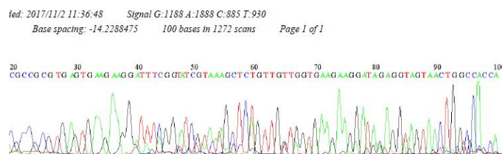
Uncultured Lactobacillus sp. clone BV_LV_OTU6489 16S ribosomal RNA gene, partial sequence Sequence ID: JQ962826.2 Length: 328 Number of Matches: 1
