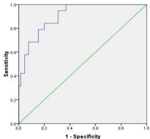
ROC Curve
