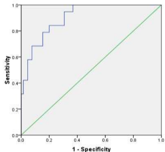
ROC Curve
