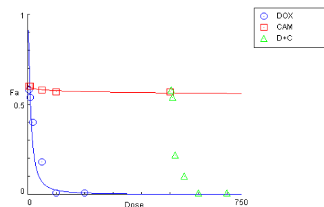
Median-Effect Plot
